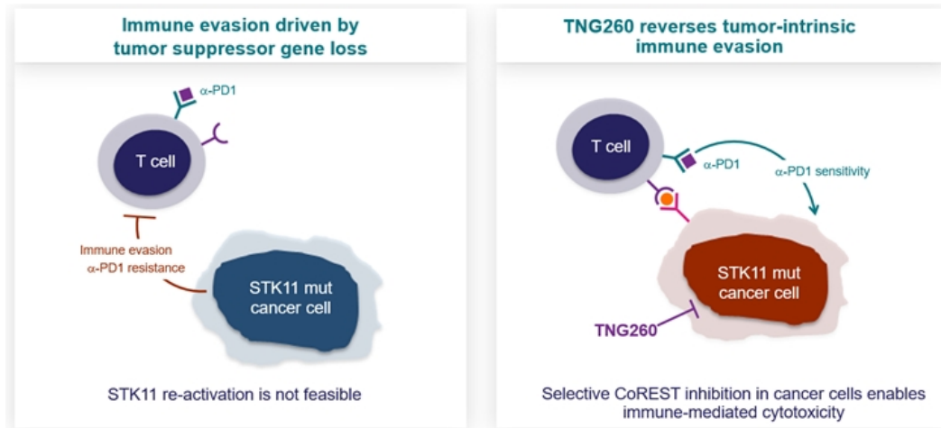
Figure 7. TNG260 mechanism of action
