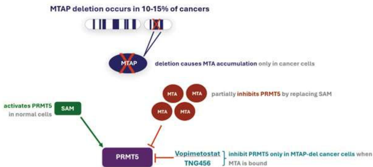
Figure 4. Vopimetostat and TNG456 have an MTA-cooperative mechanism of action that is selective for MTAP-deleted cancer cells
